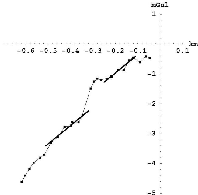
Figure 4: The data shows the gravity residuals for the Nevada U20AK borehole Airy measurements of the g(r) profile [12], defined as \Delta g(r) = g_{Newton} - g_{observed} , and measured in mGal, plotted against depth in km. This residual shows regions of linearity interspersed with regions of non-linearity, presumably arising from layers with a density different from the main density of 2000 \text{ kg/m}^3 . Density changes generate a change in the (arbitrary) residual offset. From a least-squares simultaneous fit of the linear form in (15) to the slope of the four linear regions in this data and that in Fig.5 for the data from borehole U20AL, we obtain \alpha^{-1} = 136.8 \pm 3 . The two fitted regions of data are shown by the two straight lines here and in Fig.5.
