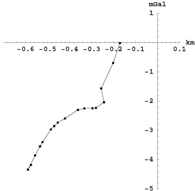
Figure 6: The data shows the gravity residuals from the third Nevada U20AO borehole Airy measurements of the g(r) profile [12]. This data is not of sufficient linearity, presumably due to non-uniformity of density, to permit a fit to the linear form in (15), but is included here for completeness. There is an arbitrary offset in the residual.
