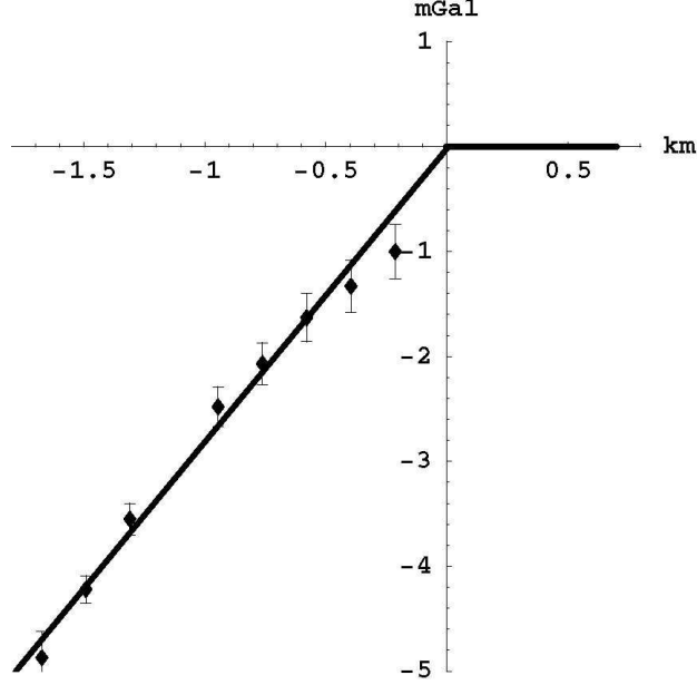
Figure 3: The data shows the gravity residuals for the Greenland Ice Shelf [11] Airy measurements of the g(r) profile, defined as \Delta g(r) = g_{Newton} - g_{observed} , and measured in mGal ( 1\text{mGal} = 10^{-3} \text{ cm/s}^2 ) and plotted against depth in km. The gravity residuals have been offset. The borehole effect is that Newtonian gravity and the new theory differ only beneath the surface, provided that the measured above surface gravity gradient is used in both theories. This then gives the horizontal line above the surface. Using (15) we obtain \alpha^{-1} = 137.9 \pm 5 from fitting the slope of the data, as shown. The non-linearity in the data arises from modelling corrections for the gravity effects of the irregular sub ice-shelf rock topography.
