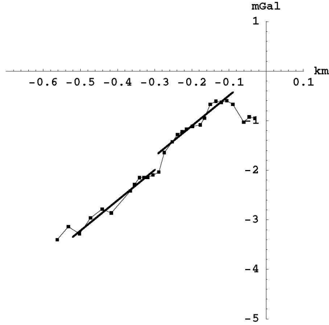
Figure 5: The data shows the gravity residuals for the Nevada U20AL borehole Airy measurements of the g(r) profile [12], defined as \Delta g(r) = g_{Newton} - g_{observed} , and measured in mGal, plotted against depth in km. This residual shows regions of linearity interspersed with regions of non-linearity, presumably arising from layers with a density different from the main density of 2000 \text{ kg/m}^3 . Density changes generate a change in the (arbitrary) residual offset. From a least-squares simultaneous fit of the linear form in (15) to the slope of the four linear regions in this data and that in Fig.4 for the data from borehole U20AK in Fig.4, we obtain \alpha^{-1} = 136.8 \pm 3 . The two fitted regions of data are shown by the two straight lines here and in Fig.4.
