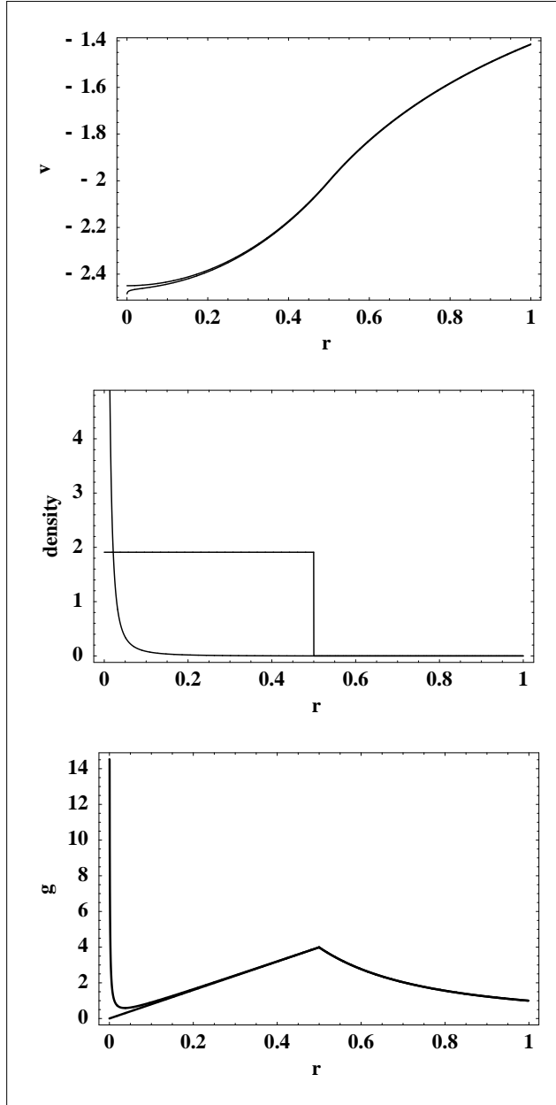
Figure 1: Upper plot shows speeds from numerical iterative solution of (7) for a solid sphere with uniform density and radius r = 1 for (i) upper curve the case \alpha = 0 corresponding to Newtonian gravity, and (ii) lower curve with \alpha = 1/137 . These solutions only differ significantly near r = 0 . Middle plot shows matter density and ‘dark matter’ density \rho_{DM} , from (5), with arbitrary scales. Lower plot shows the acceleration from (3) for (i) the Newtonian in-flow from the upper plot, and (ii) from the \alpha = 1/137 case. The difference is only significant near r = 0 . The accelerations begin to differ just inside the surface of the sphere at r = 1 , according to (15). This difference is the origin of the borehole g anomaly, and permits the determination of the value of \alpha from observational data. This generic singular- g behaviour, at r = 0 , is seen in the earth, in globular clusters and in galaxies.
