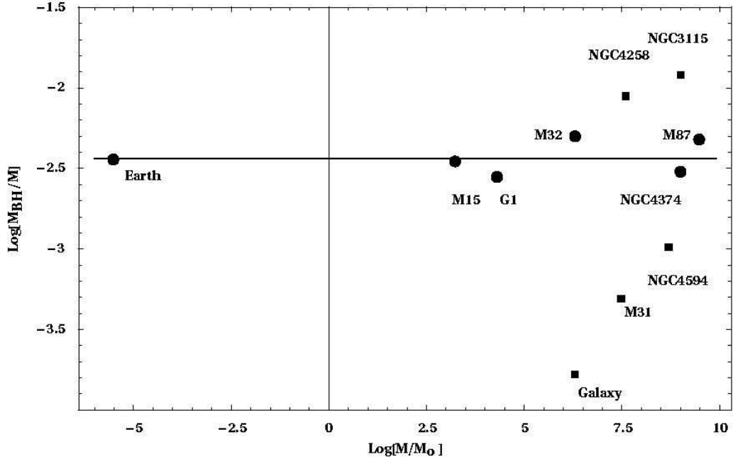
Figure 2: The data shows \text{Log}_{10}[M_{BH}/M] for the ‘blackhole’ or ‘dark matter’ masses M_{BH} for a variety of spherical matter systems with masses M , shown by solid circles, plotted against \text{Log}_{10}[M/M_0] , where M_0 is the solar mass, showing agreement with the ‘ \alpha/2 -line’ ( \text{Log}_{10}[\alpha/2] = -2.44 ) predicted by (10), and ranging over 15 orders of magnitude. The ‘blackhole’ effect is the same phenomenon as the ‘dark matter’ effect. The data ranges from the earth, as observed by the bore hole g anomaly, to globular cluster M15 and G1, and then to spherical ‘elliptical’ galaxies M32 (E2), NGC 4374 (E1) and M87 (E0). Best fit to the data from these star systems gives \alpha = 1/134 , while for the earth data in Figs.3, 4, 5 give \alpha = 1/137 . In these systems the ‘dark matter’ or ‘black hole’ spatial self-interaction effect is induced by the matter. For the spiral galaxies, shown by the filled boxes, where here M is the bulge mass, the blackhole masses do not correlate with the ‘ \alpha/2 -line’. This is because these systems form by matter in-falling to a primordial blackhole, and so these systems are more contingent. For spiral galaxies this dynamical effect manifests most clearly via the non-Keplerian rotation-velocity curve, which decrease asymptotically very slowly. See [7] for references to the data.
