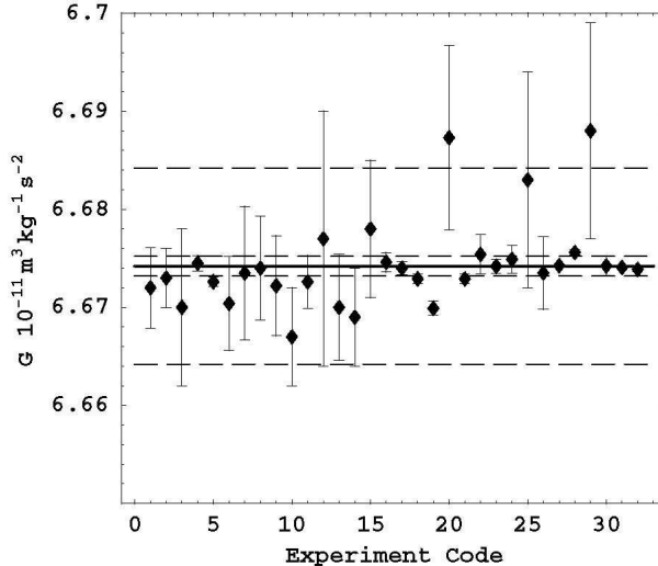
Figure 7: Results of precision measurements of G_N published in the last sixty years in which the Newtonian theory was used to analyse the data. These results show the presence of a systematic effect, not in the Newtonian theory, of fractional size up to \Delta G_N/G_N \approx \alpha/4 , which corresponded with the 1998 error bars on G_N (outer dashed lines), with the full line being the current CODATA value of G_N = (6.6742(10) \times 10^{-11} \text{ m}^2\text{s}^{-2}\text{kg}^{-1}) . In 2005 CODATA [20] reduced the error bars by a factor of 10 (inner dashed lines) on the basis of some recent experiments, and so neglecting the presence of the systematic effect.
